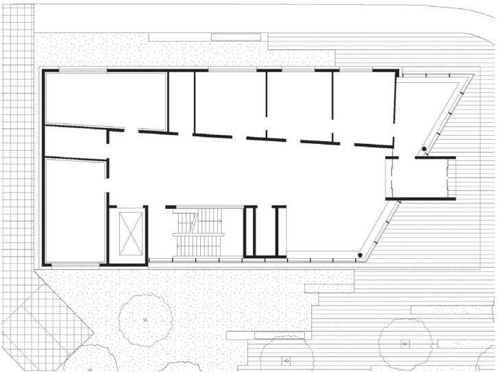
Ground Plan, ground floor
